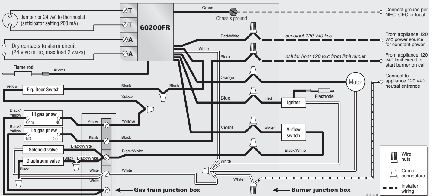
Figure 11 Wiring diagram — 301GAS burner with 60200FR primary control (Replaces Figure 11, page 11)
